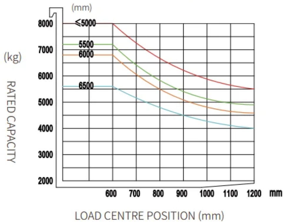
EFL803-HV-6 RATED CAPACITIES AND LOAD CENTERES GRAPH
